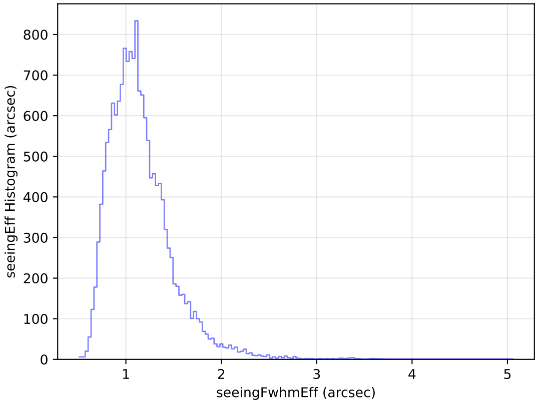
ddf_loaded_fl4_v3.4_10yrs Yr 1 u band: seeingEff Histogram
