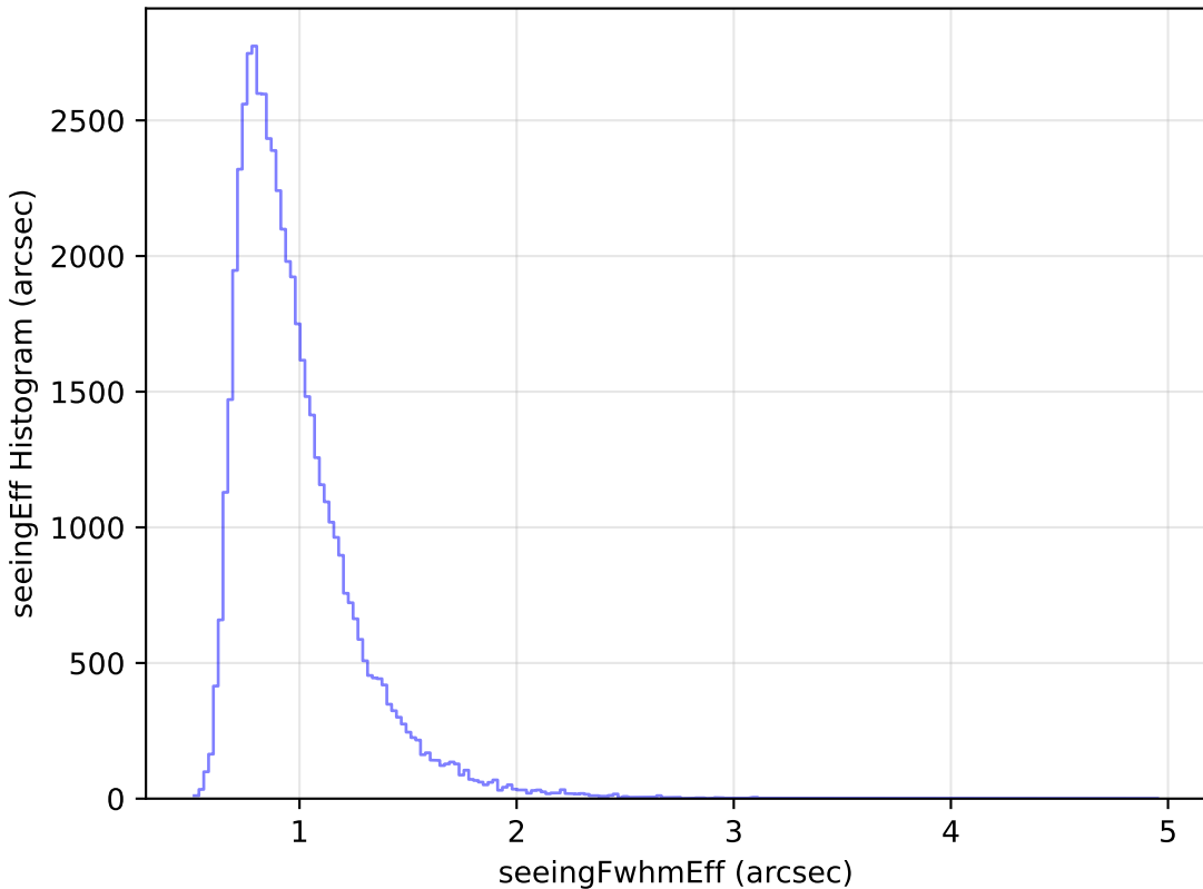
ddf_loaded_fl4_v3.4_10yrs Yr 1 i band: seeingEff Histogram
