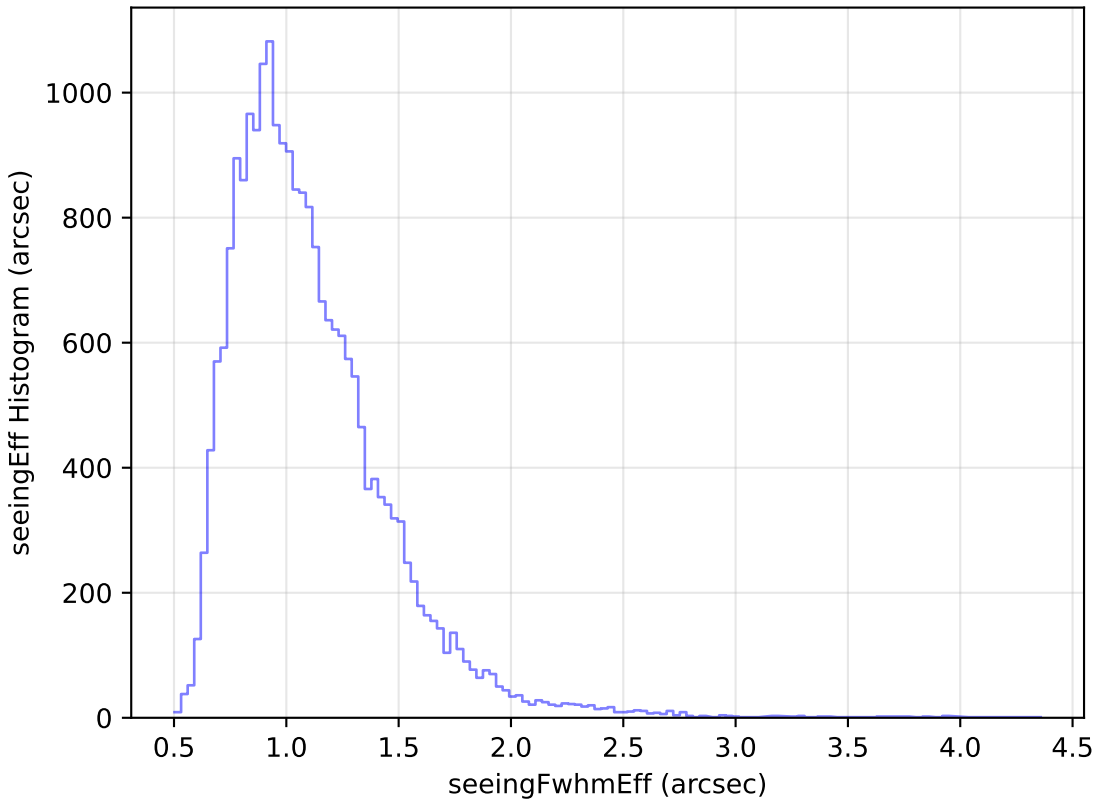
ddf_loaded_fl4_v3.4_10yrs Yr 1 g band: seeingEff Histogram
