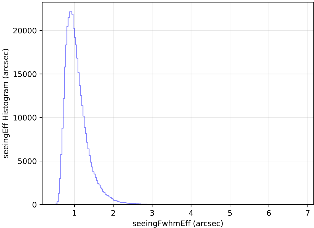
ddf_loaded_fl4_v3.4_10yrs WFD y band: seeingEff Histogram
