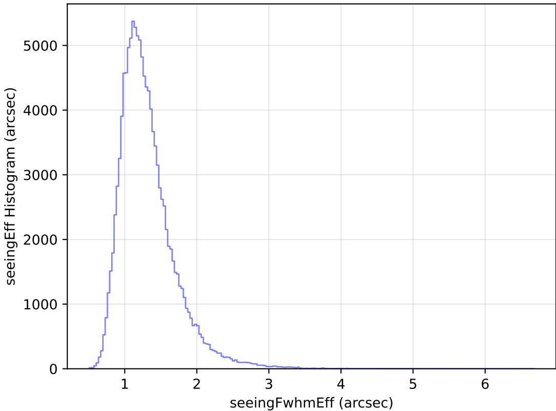
ddf_loaded_fl4_v3.4_10yrs WFD u band: seeingEff Histogram
