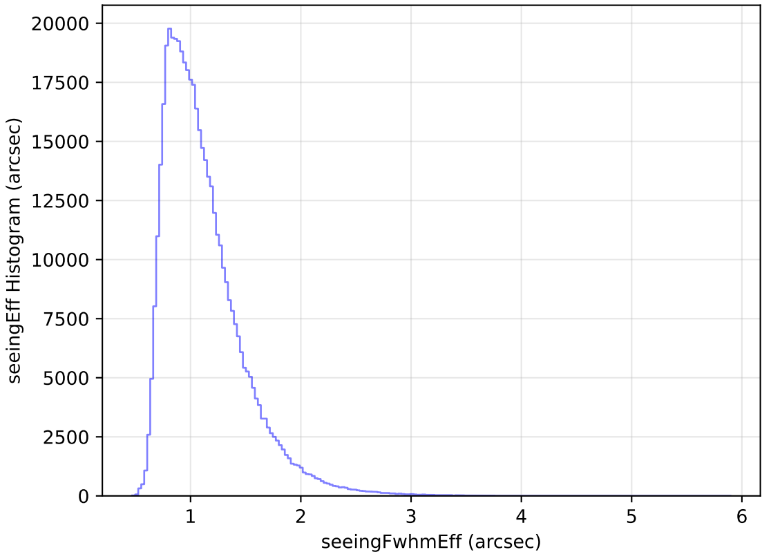
ddf_loaded_fl4_v3.4_10yrs WFD r band: seeingEff Histogram
