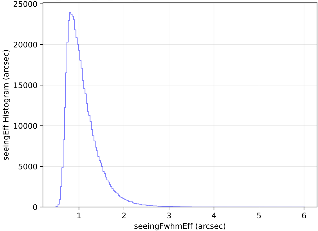
ddf_loaded_fl4_v3.4_10yrs WFD i band: seeingEff Histogram
