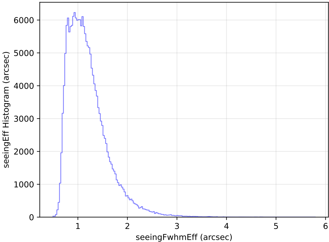
ddf_loaded_fl4_v3.4_10yrs WFD g band: seeingEff Histogram
