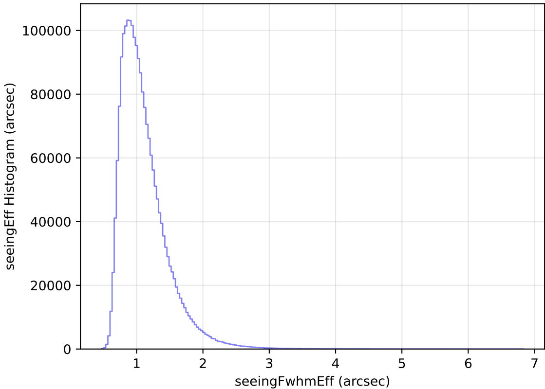
ddf_loaded_fl4_v3.4_10yrs WFD all bands: seeingEff Histogram
