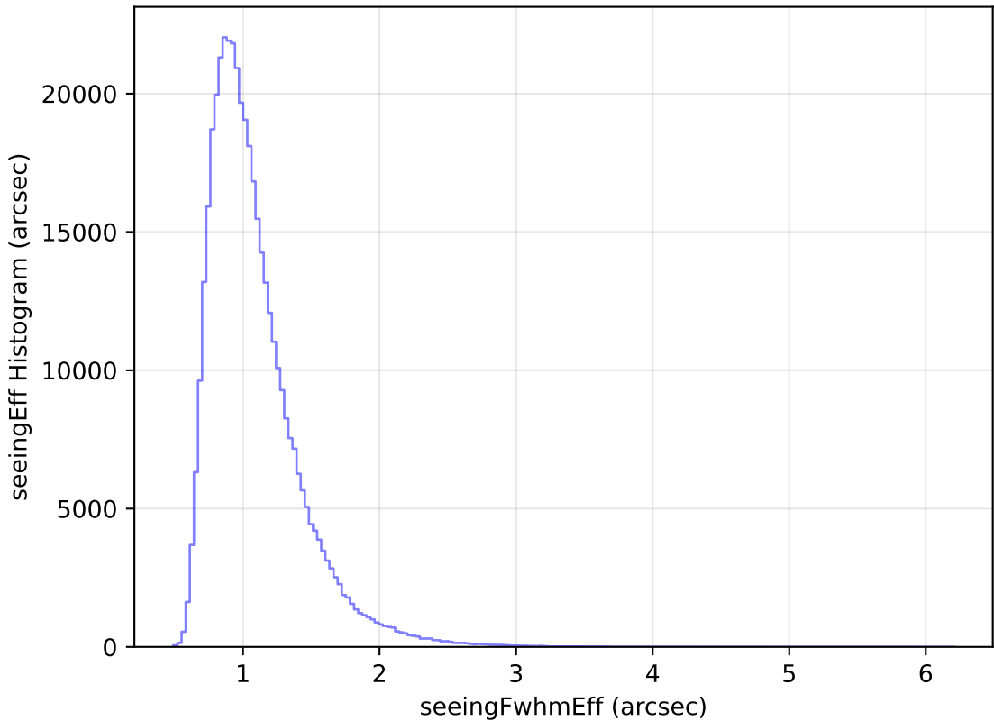
ddf_loaded_fl4_v3.4_10yrs All sky z band: seeingEff Histogram
