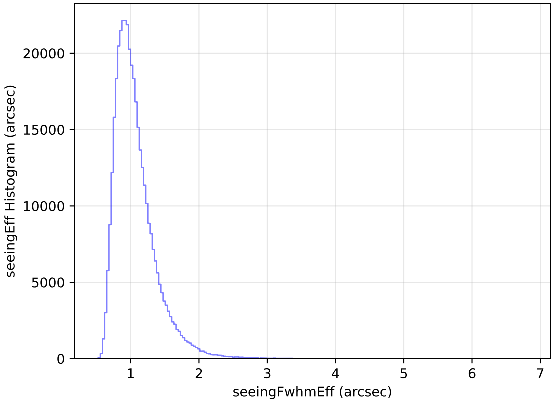
ddf_loaded_fl4_v3.4_10yrs All sky y band: seeingEff Histogram
