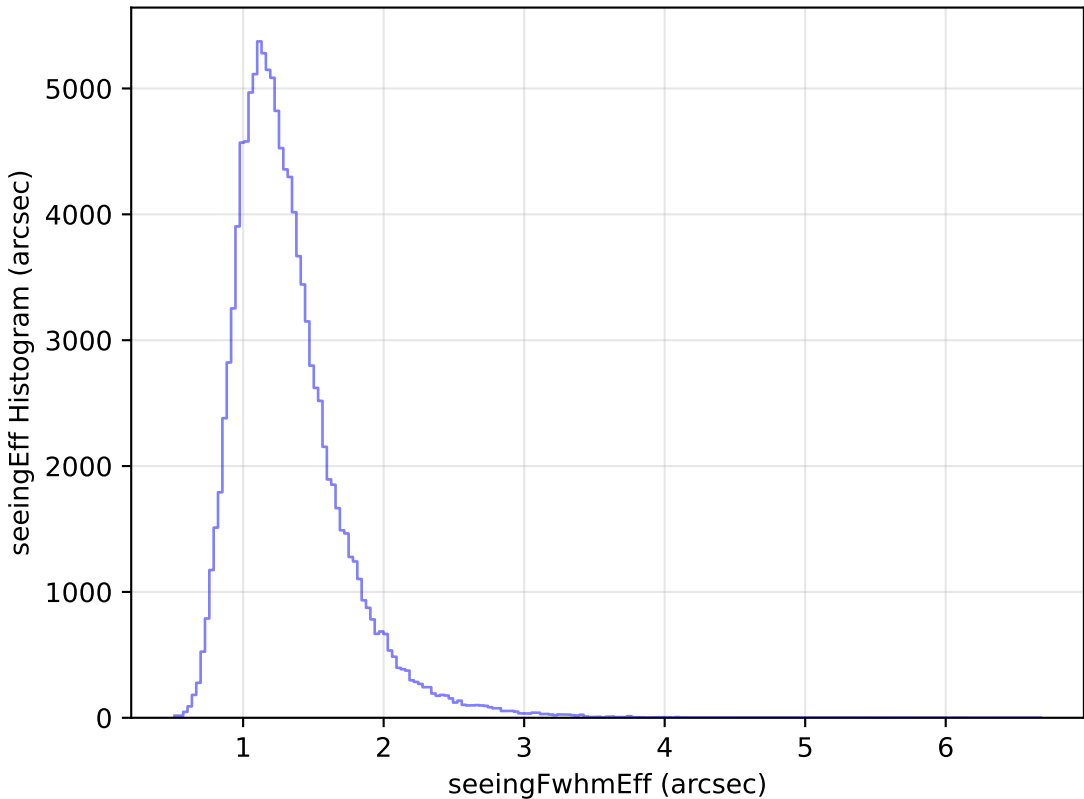
ddf_loaded_fl4_v3.4_10yrs All sky u band: seeingEff Histogram
