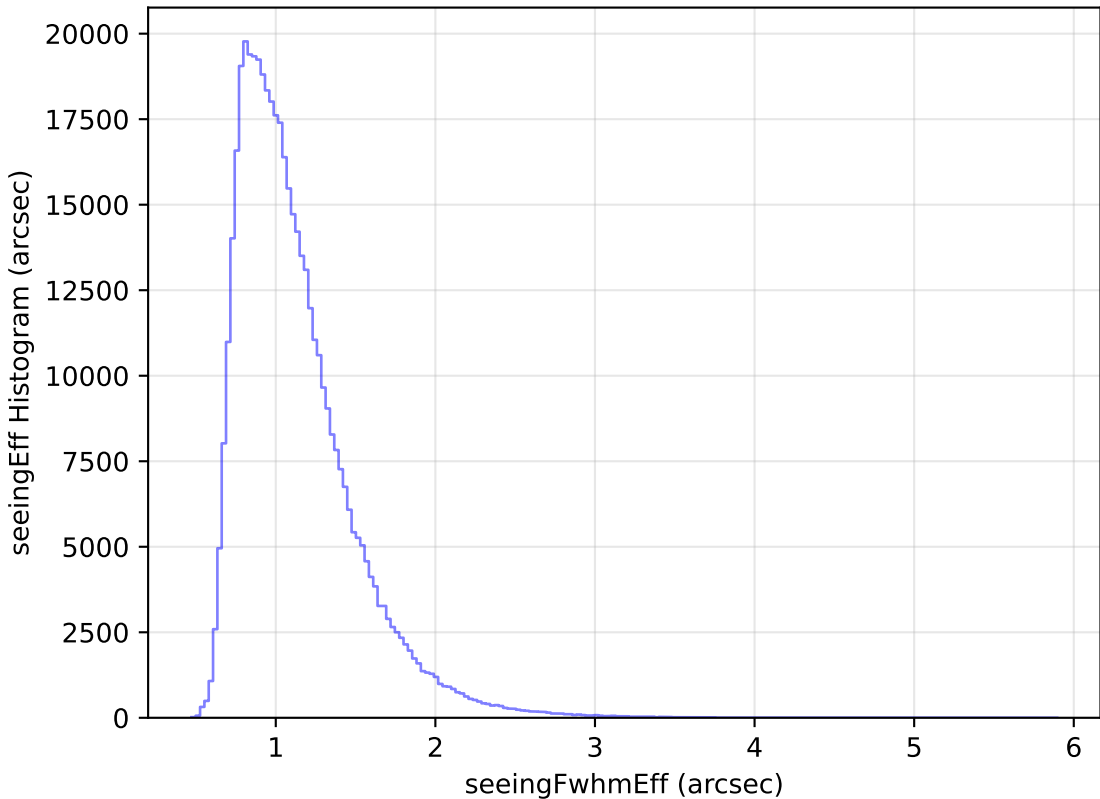
ddf_loaded_fl4_v3.4_10yrs All sky r band: seeingEff Histogram
