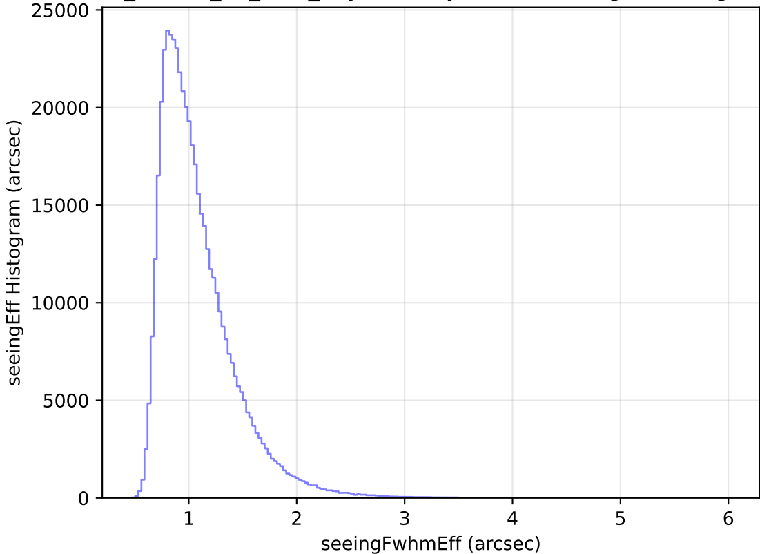
ddf_loaded_fl4_v3.4_10yrs All sky i band: seeingEff Histogram
