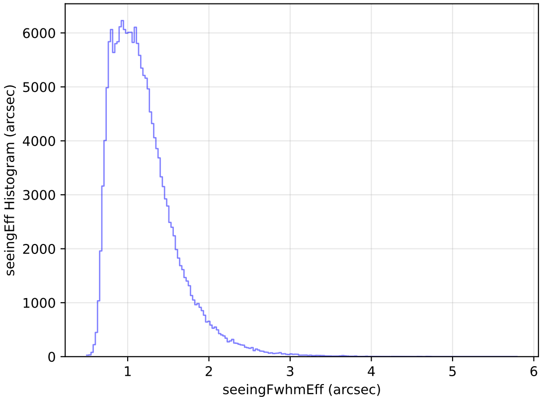
ddf_loaded_fl4_v3.4_10yrs All sky g band: seeingEff Histogram
