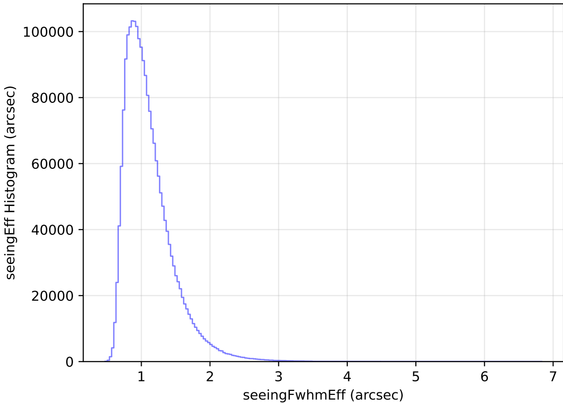
ddf_loaded_fl4_v3.4_10yrs All sky all bands: seeingEff Histogram
