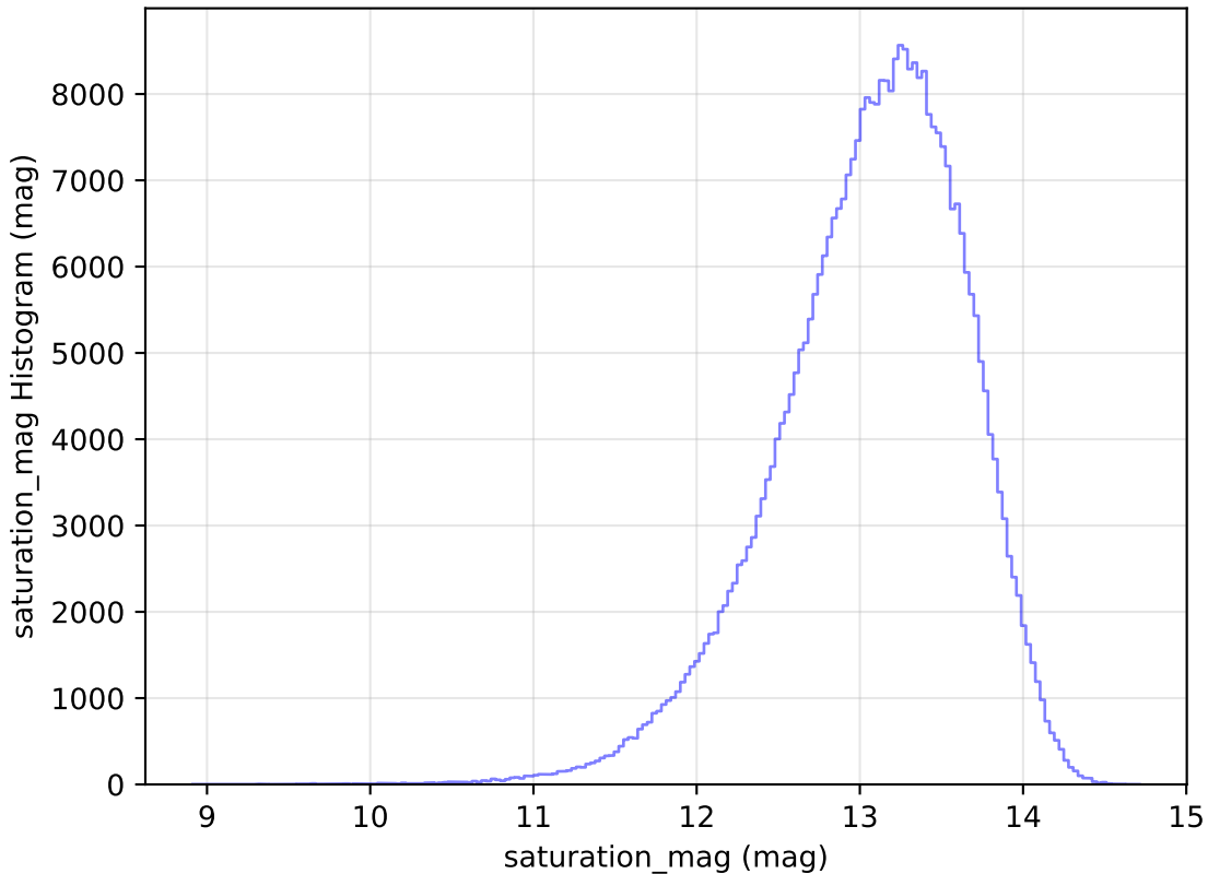
ddf_loaded_fl4_v3.4_10yrs WFD y band: saturation_mag Histogram
