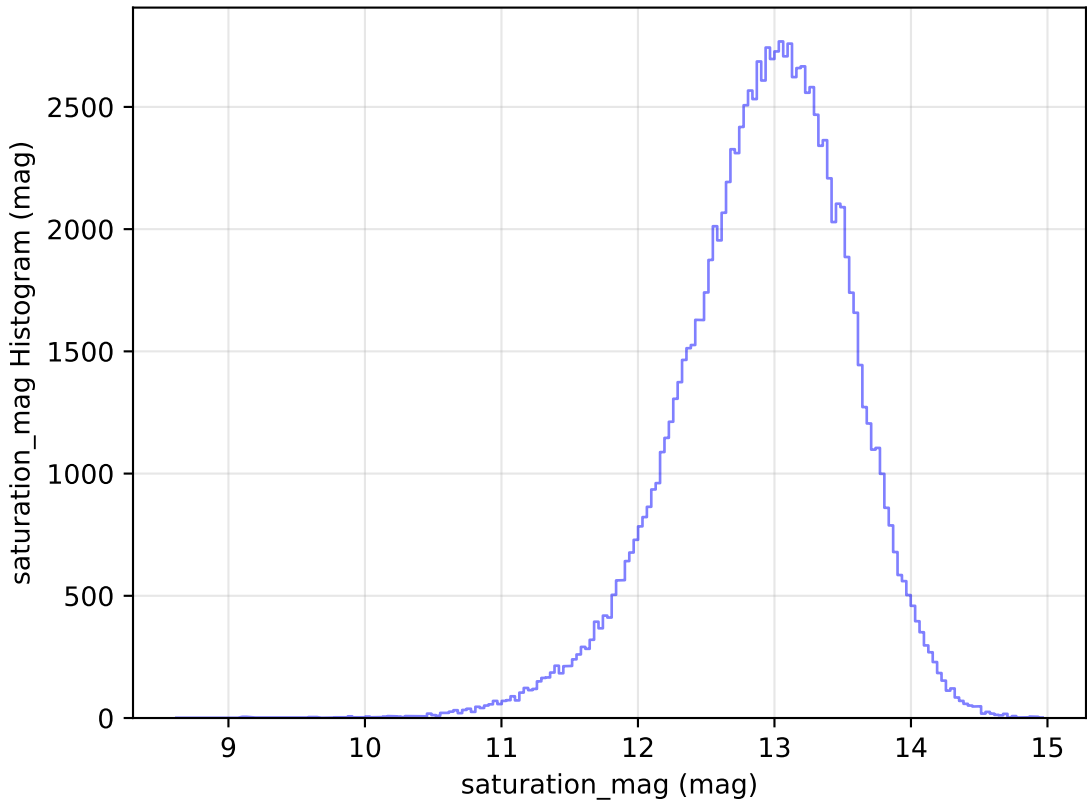
ddf_loaded_fl4_v3.4_10yrs WFD u band: saturation_mag Histogram
