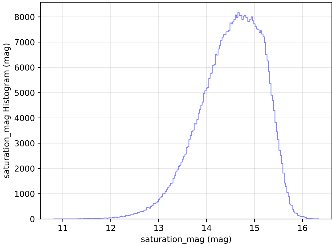
ddf_loaded_fl4_v3.4_10yrs WFD r band: saturation_mag Histogram
