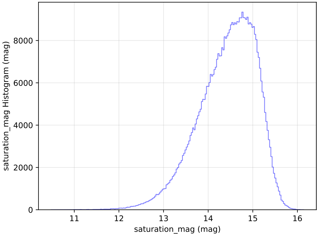
ddf_loaded_fl4_v3.4_10yrs WFD i band: saturation_mag Histogram
