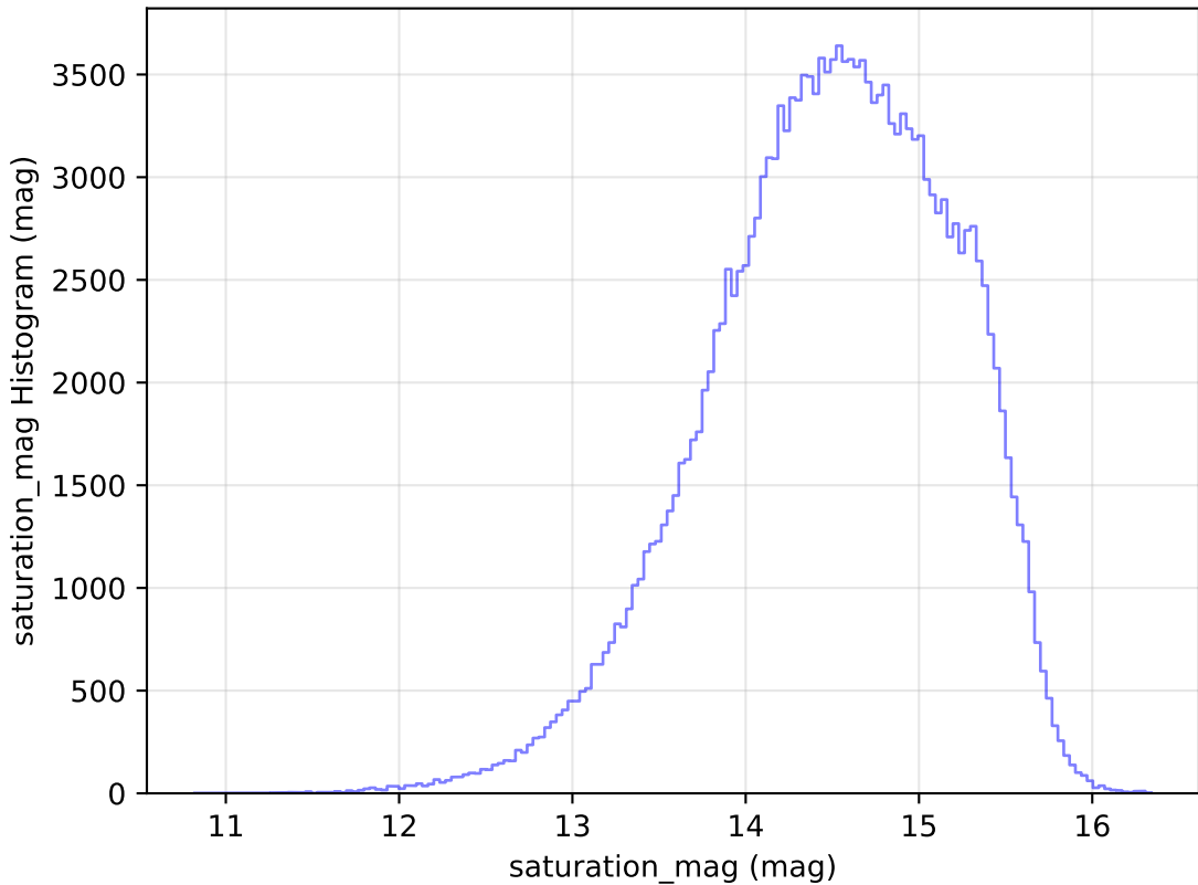
ddf_loaded_fl4_v3.4_10yrs WFD g band: saturation_mag Histogram
