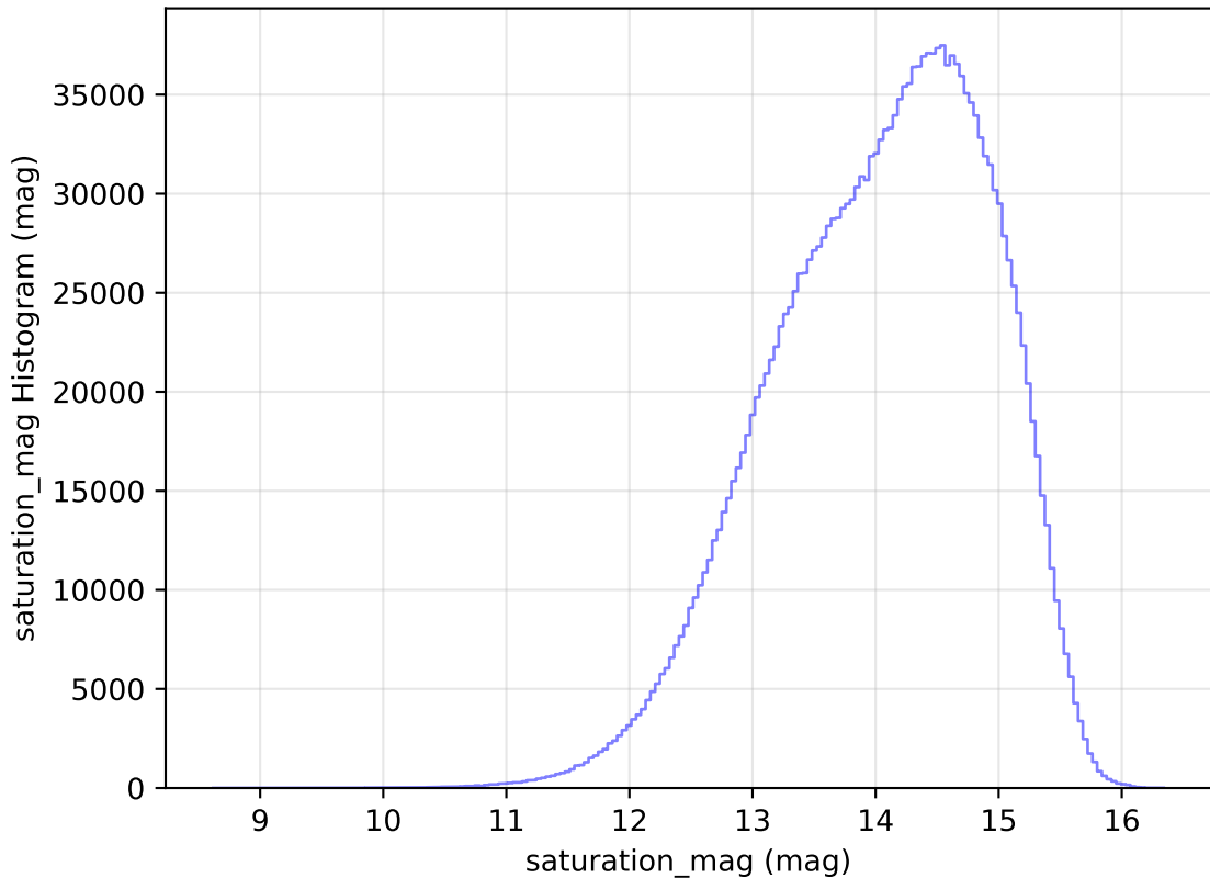
ddf_loaded_fl4_v3.4_10yrs WFD all bands: saturation_mag Histogram
