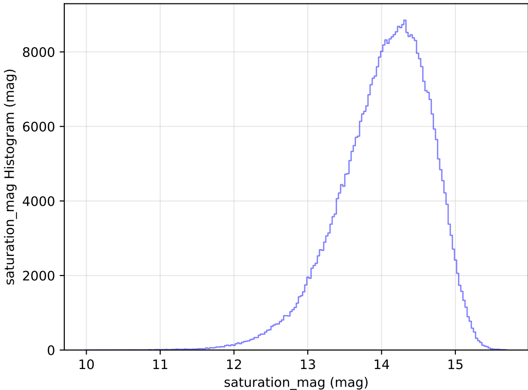
ddf_loaded_fl4_v3.4_10yrs All sky z band: saturation_mag Histogram
