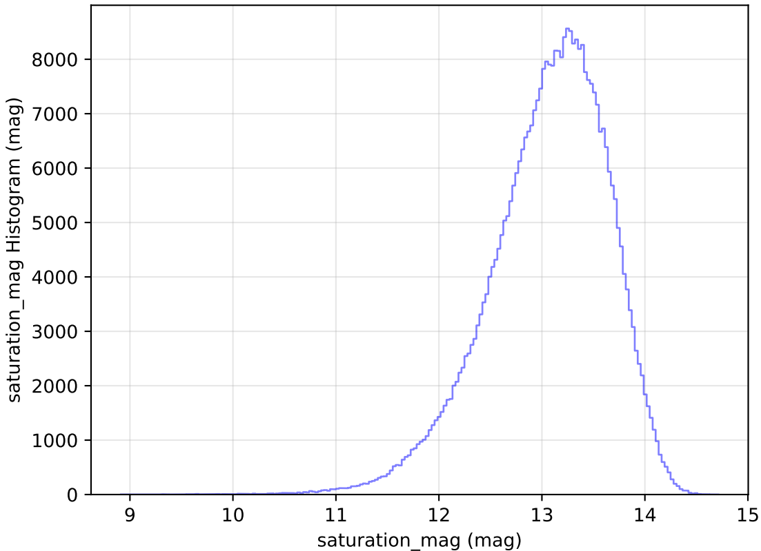
ddf_loaded_fl4_v3.4_10yrs All sky y band: saturation_mag Histogram
