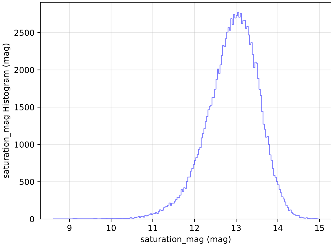
ddf_loaded_fl4_v3.4_10yrs All sky u band: saturation_mag Histogram
