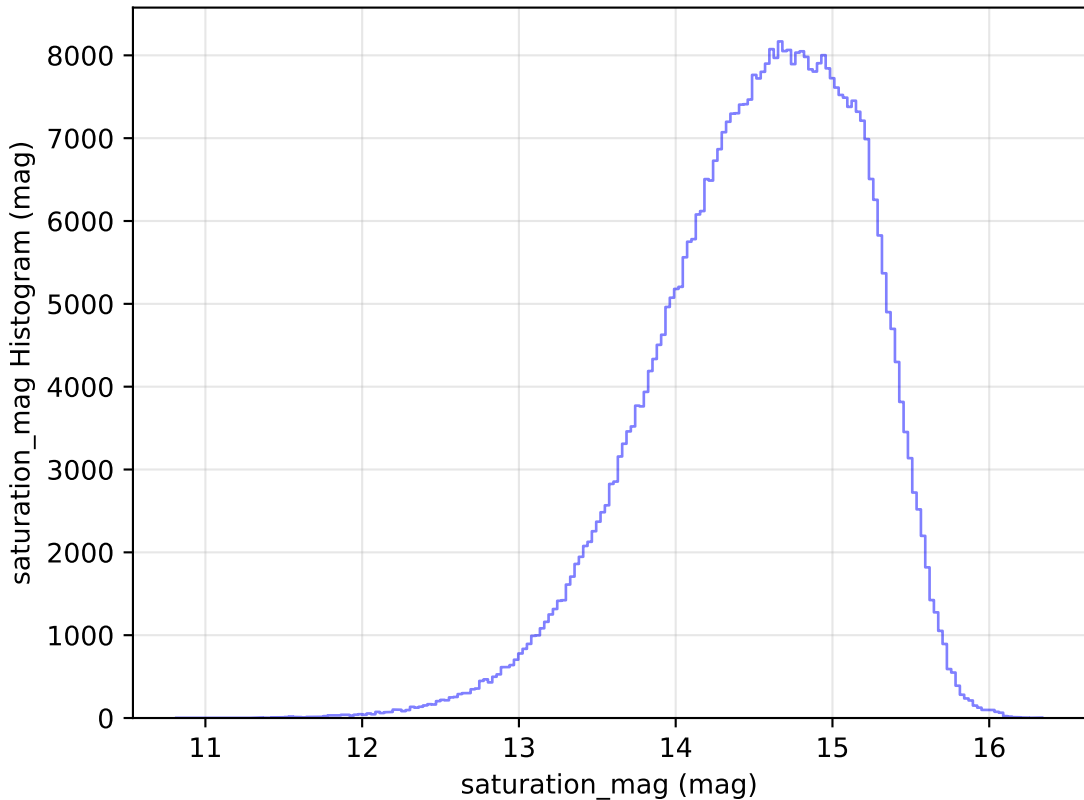
ddf_loaded_fl4_v3.4_10yrs All sky r band: saturation_mag Histogram
