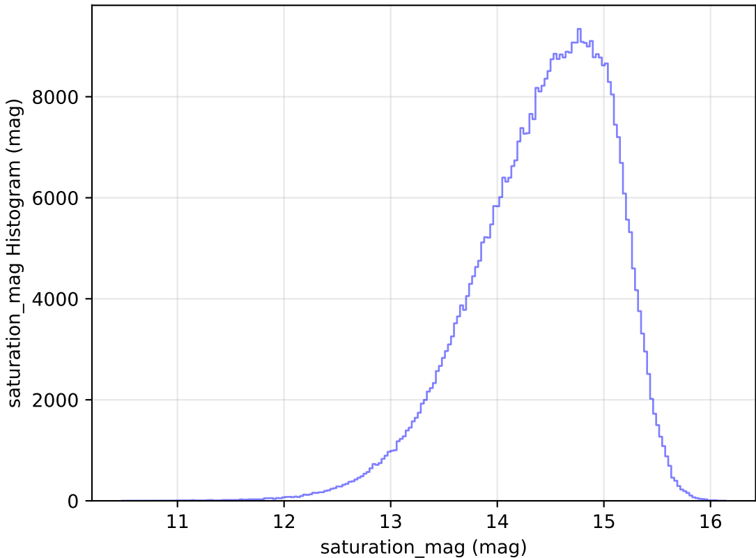
ddf_loaded_fl4_v3.4_10yrs All sky i band: saturation_mag Histogram
