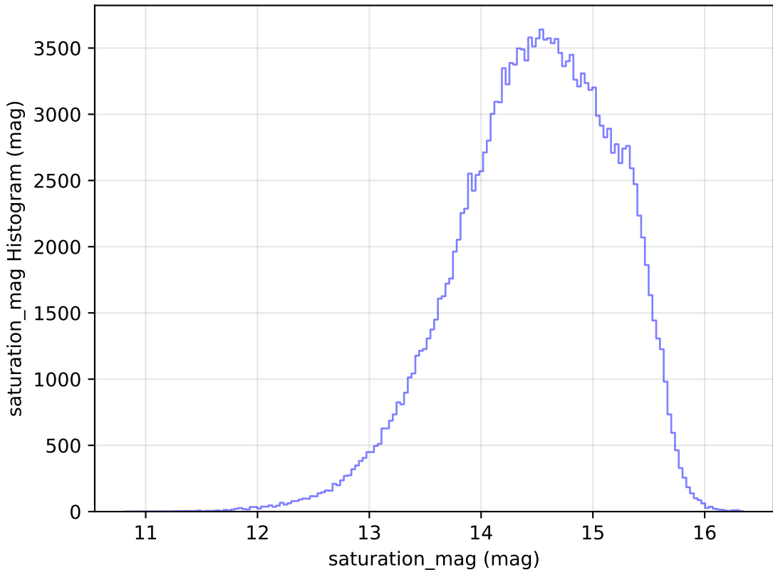
ddf_loaded_fl4_v3.4_10yrs All sky g band: saturation_mag Histogram
