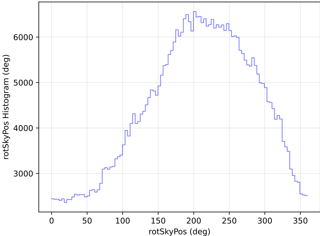
ddf_loaded_fl4_v3.4_10yrs WFD z band: rotSkyPos Histogram
