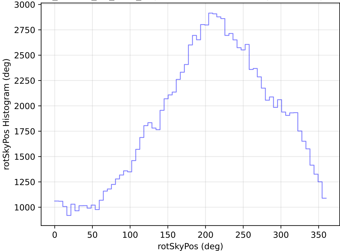
ddf_loaded_fl4_v3.4_10yrs WFD u band: rotSkyPos Histogram
