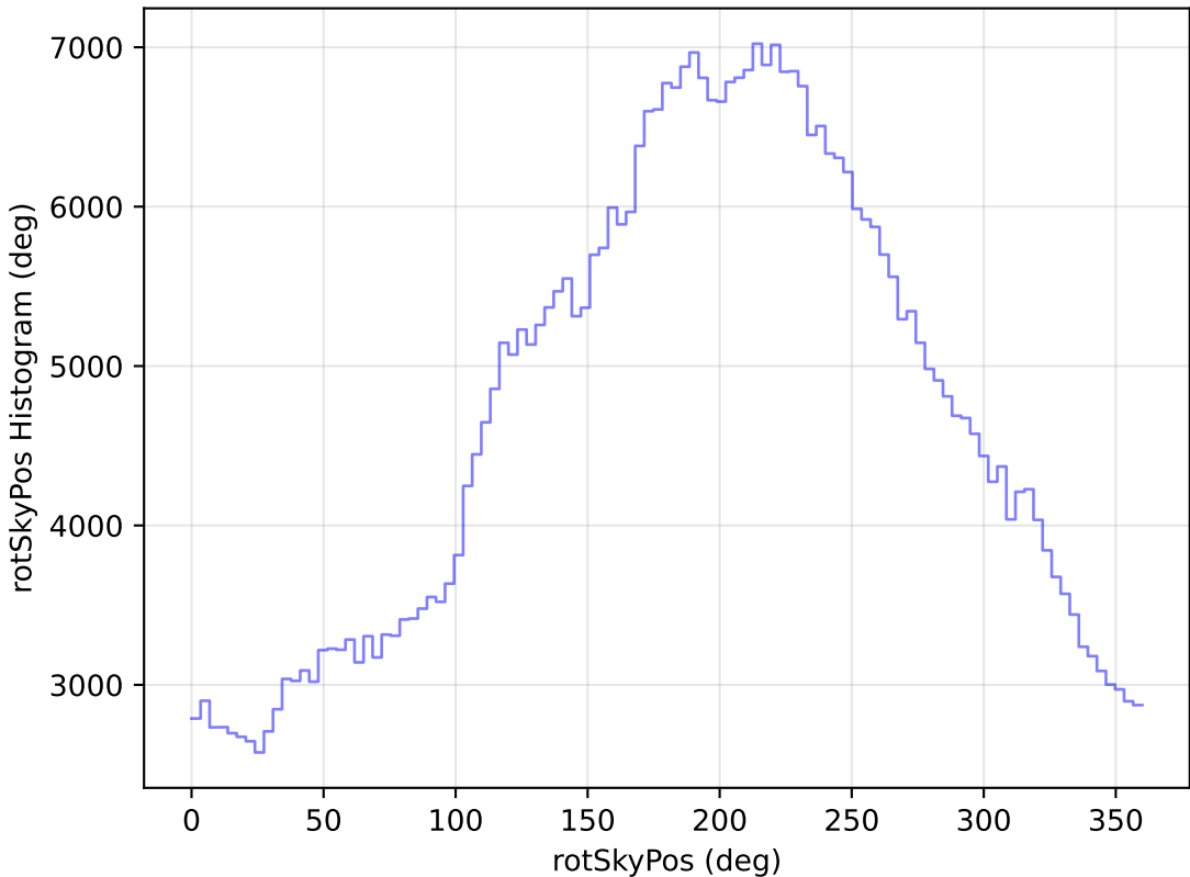
ddf_loaded_fl4_v3.4_10yrs WFD r band: rotSkyPos Histogram
