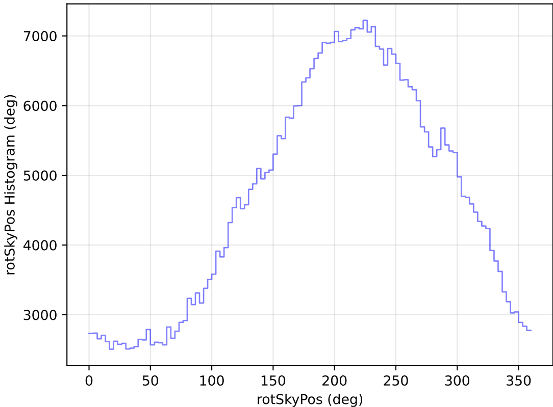
ddf_loaded_fl4_v3.4_10yrs WFD i band: rotSkyPos Histogram
