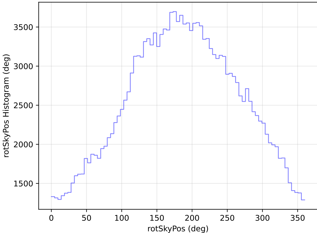
ddf_loaded_fl4_v3.4_10yrs WFD g band: rotSkyPos Histogram
