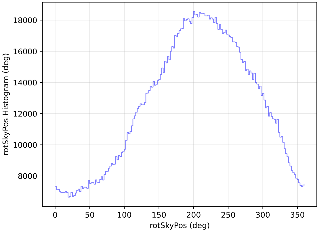
ddf_loaded_fl4_v3.4_10yrs WFD all bands: rotSkyPos Histogram
