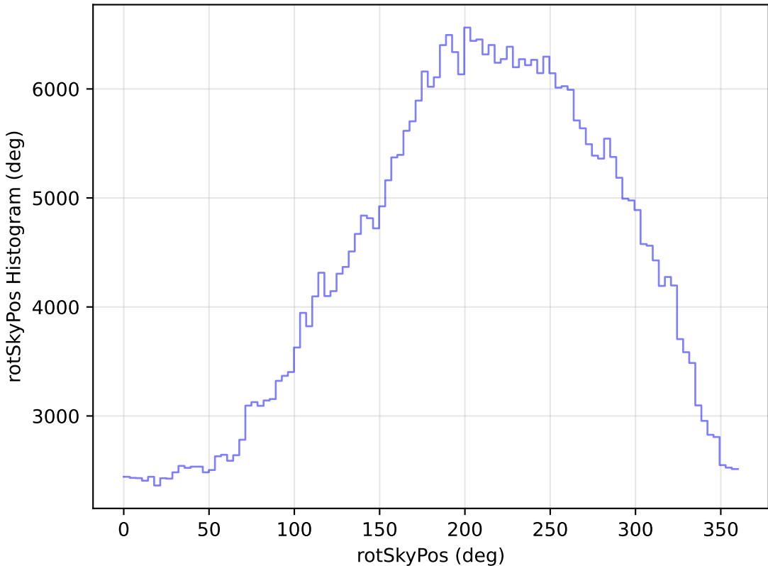
ddf_loaded_fl4_v3.4_10yrs All sky z band: rotSkyPos Histogram
