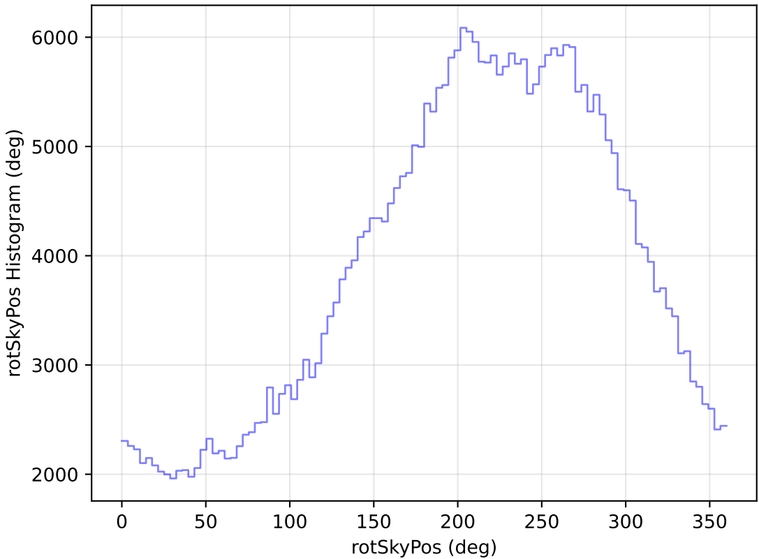
ddf_loaded_fl4_v3.4_10yrs All sky y band: rotSkyPos Histogram
