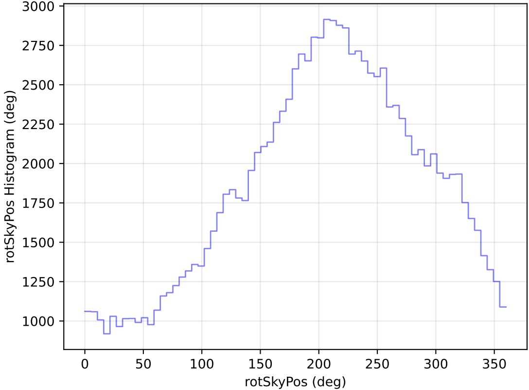
ddf_loaded_fl4_v3.4_10yrs All sky u band: rotSkyPos Histogram
