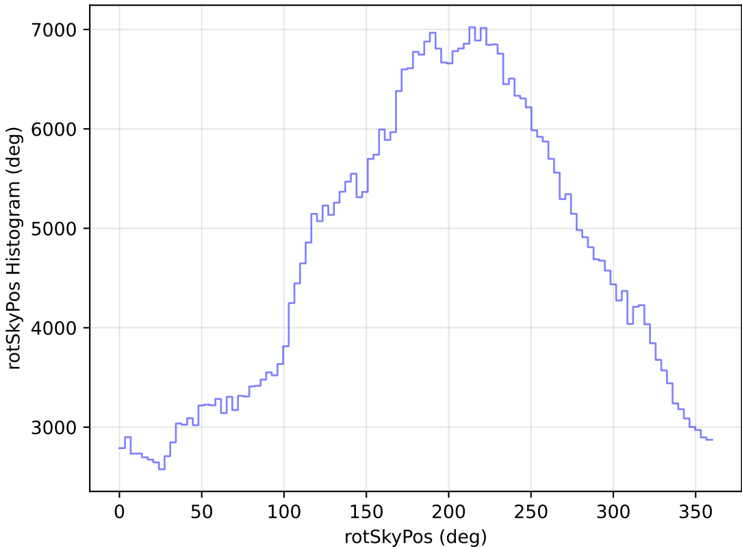
ddf_loaded_fl4_v3.4_10yrs All sky r band: rotSkyPos Histogram
