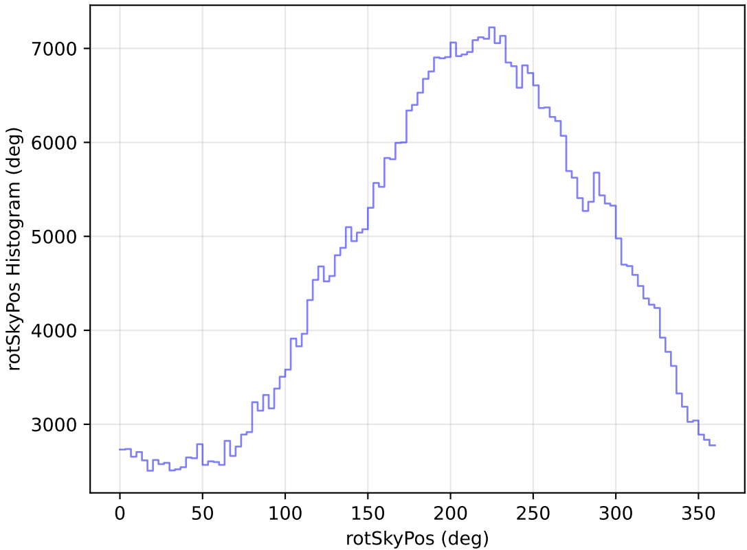
ddf_loaded_fl4_v3.4_10yrs All sky i band: rotSkyPos Histogram
