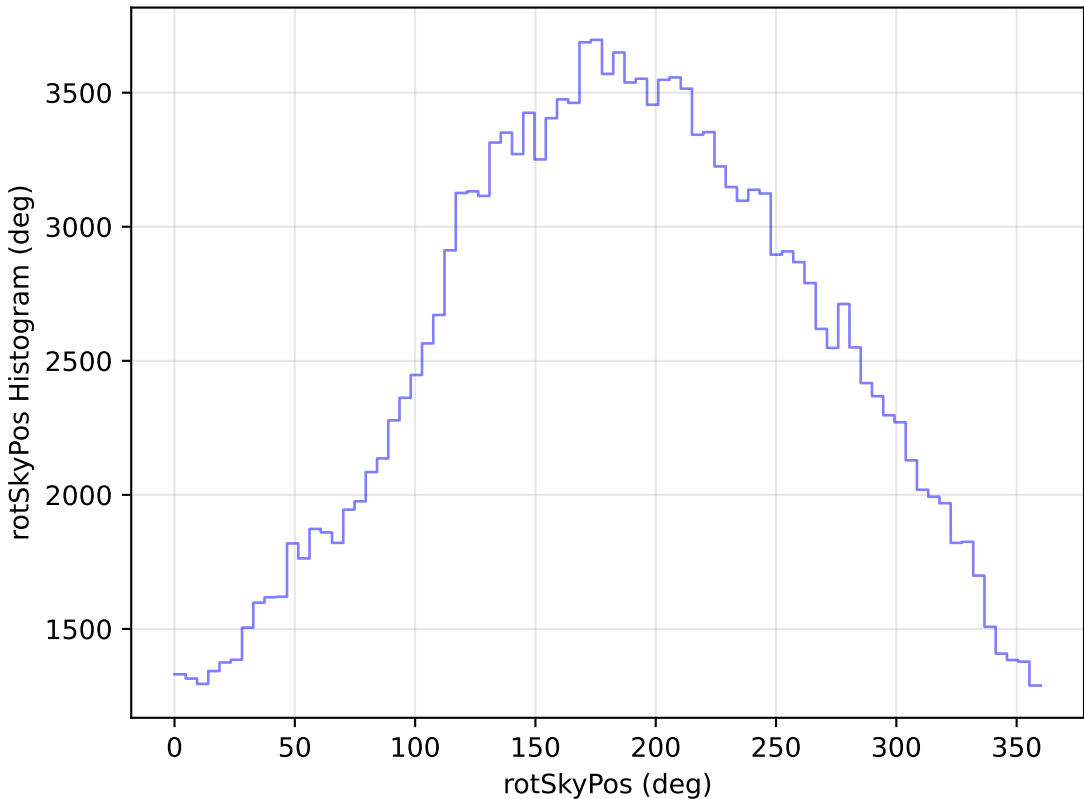
ddf_loaded_fl4_v3.4_10yrs All sky g band: rotSkyPos Histogram
