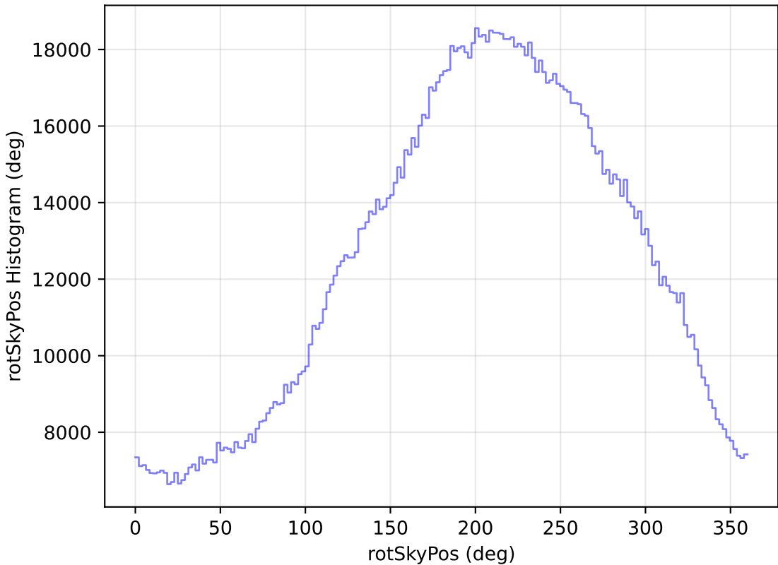
ddf_loaded_fl4_v3.4_10yrs All sky all bands: rotSkyPos Histogram
