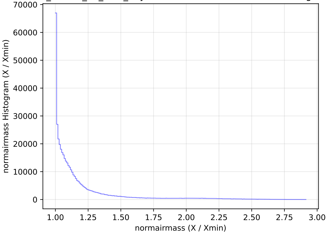
ddf_loaded_fl4_v3.4_10yrs WFD z band: normairmass Histogram
