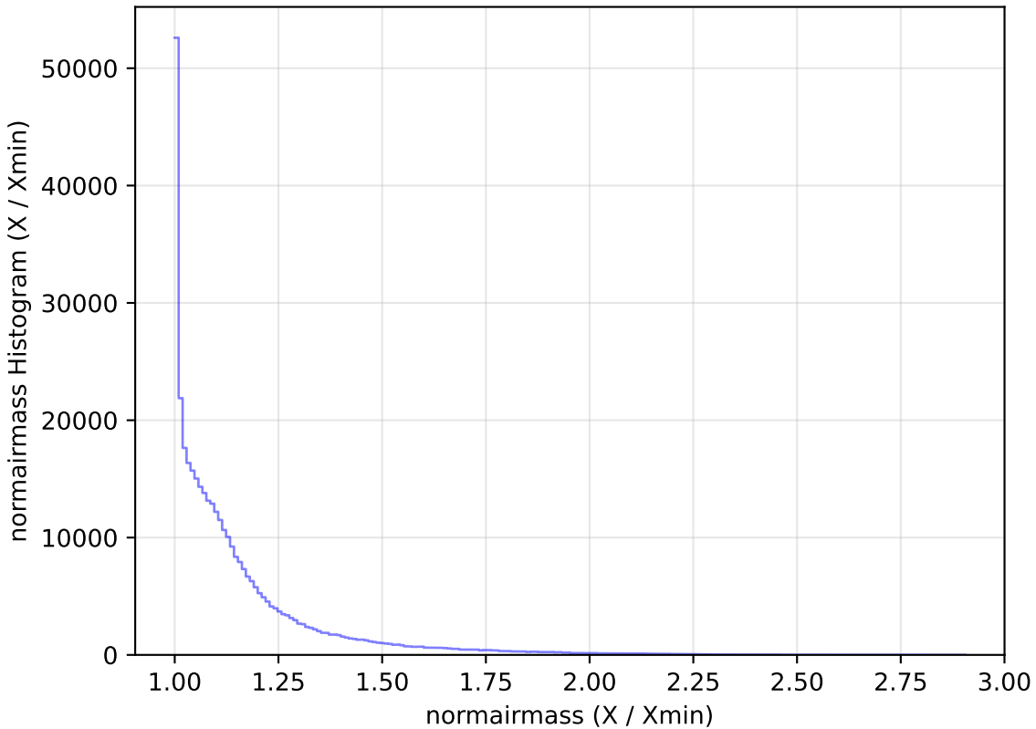
ddf_loaded_fl4_v3.4_10yrs WFD y band: normairmass Histogram
