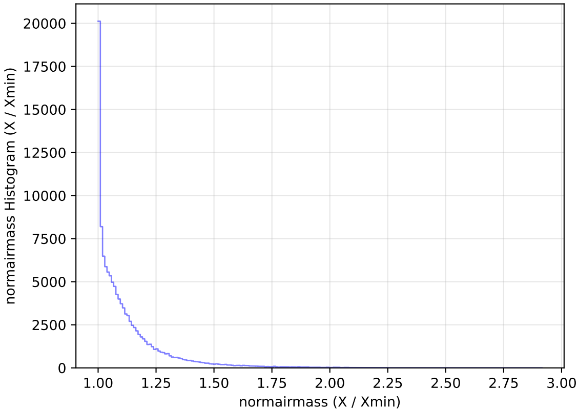
ddf_loaded_fl4_v3.4_10yrs WFD u band: normairmass Histogram
