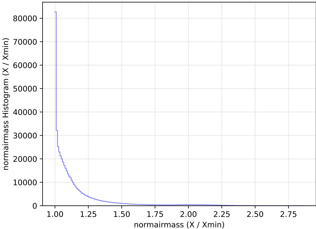
ddf_loaded_fl4_v3.4_10yrs WFD r band: normairmass Histogram
