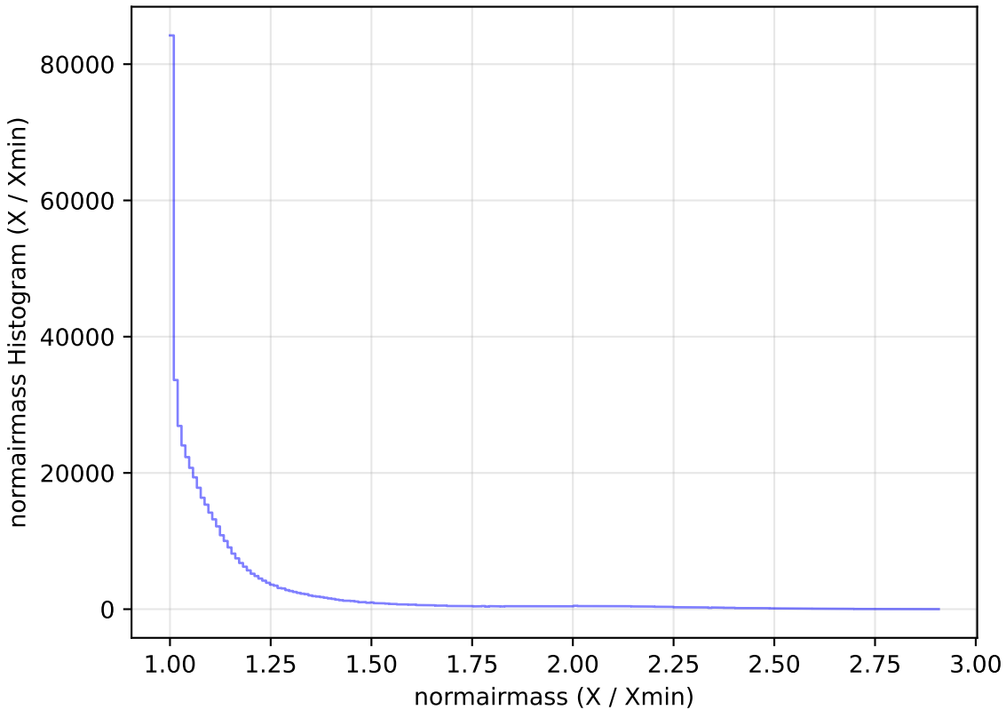
ddf_loaded_fl4_v3.4_10yrs WFD i band: normairmass Histogram
