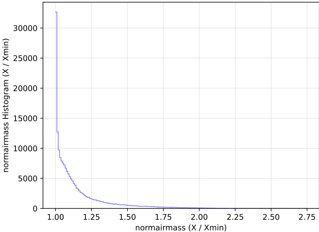
ddf_loaded_fl4_v3.4_10yrs WFD g band: normairmass Histogram
