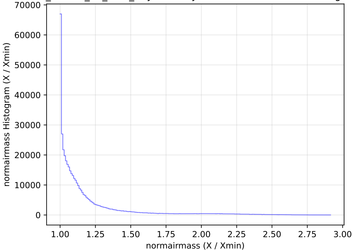
ddf_loaded_fl4_v3.4_10yrs All sky z band: normairmass Histogram
