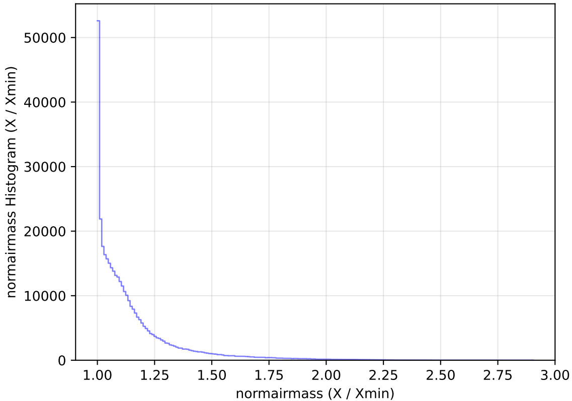
ddf_loaded_fl4_v3.4_10yrs All sky y band: normairmass Histogram
