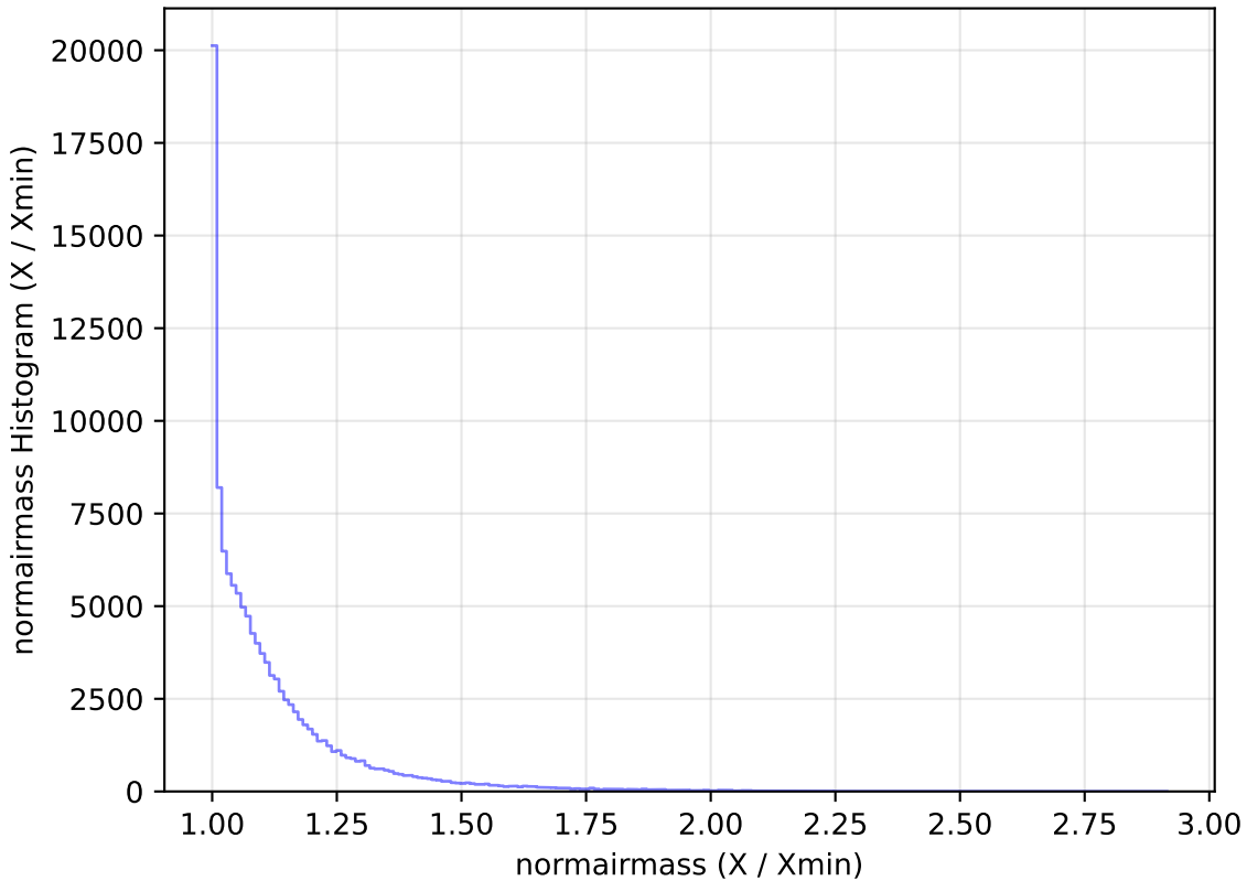
ddf_loaded_fl4_v3.4_10yrs All sky u band: normairmass Histogram
